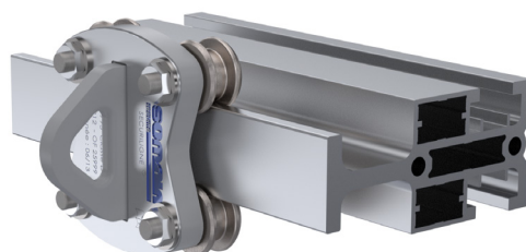
Face-fixed application
